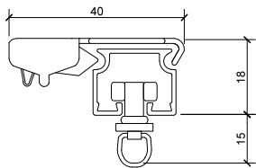
SERIES 52 Ceiling Bracket No 5153L
